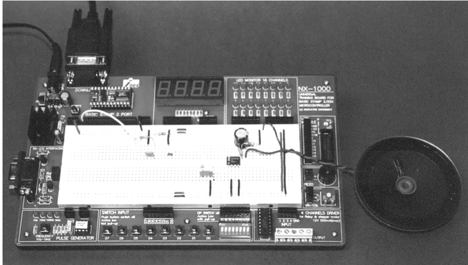
Figure 67.2: INEX-1000 laboratory
