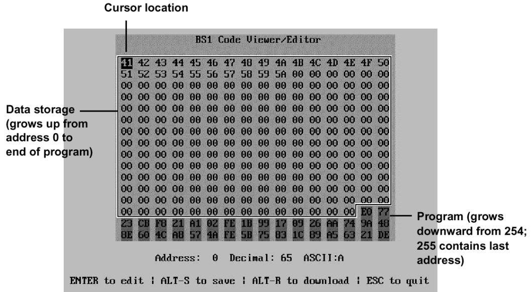
Figure 17.1. Screen shot of BS1 object-code browser graphically illustrates how the Stamp stores data and programs in EEPROM.
