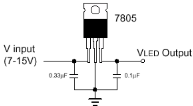
Figure 19.3: Voltage regulator for VLED
