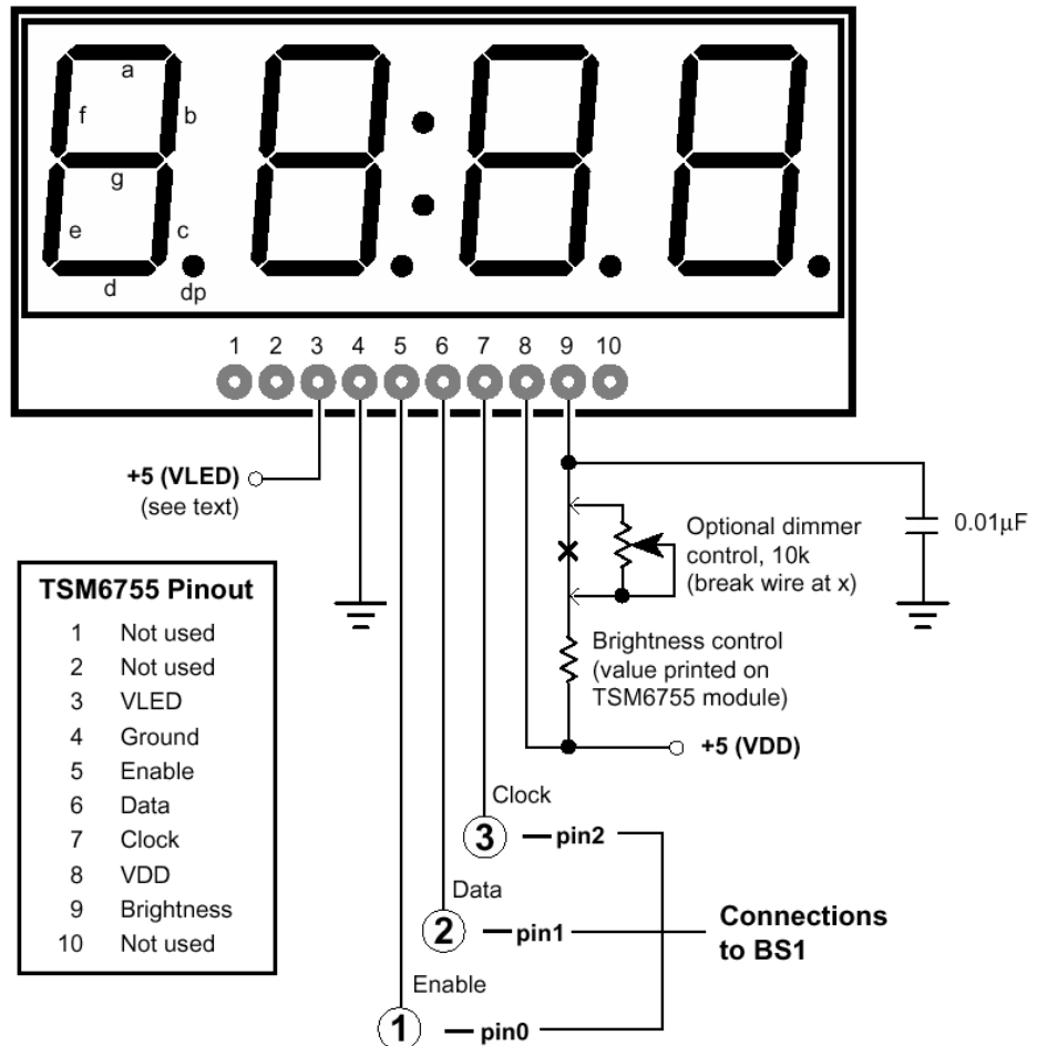
Figure 19.2: Connecting the TSM6755 LED display module.
