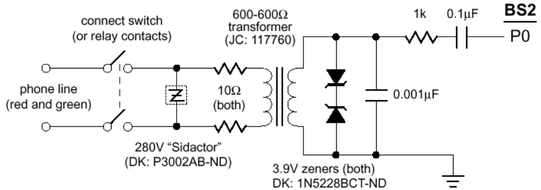
Figure 19.1: Phoneline interface for the BS2
