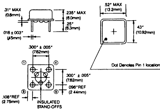
8PIN DIP
